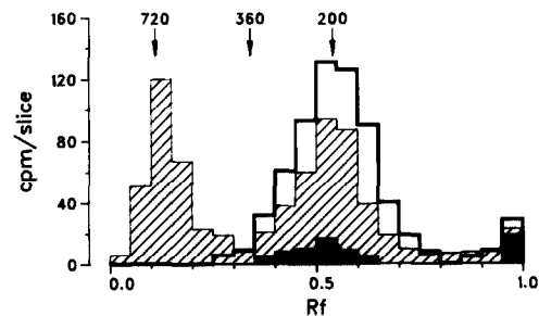
Fig.1. Cross-linking of 125 I- \alpha_1 I 3 -chymotrypsin to placental membranes. Membranes (300 \mu g protein/ml) were incubated for 18 h at 4°C with about 20 pM 125 I- \alpha_1 I 3 -chymotrypsin in the absence (open and hatched bars) or presence (filled bars) of 200 nM unlabelled \alpha_2 MT. DSS dissolved in DMSO was added to 0.2 mM and the incubation continued for 10 min (hatched and filled bars). The open bars (heavy line) show the result of the addition of DMSO only. The membranes were layered upon 60 mM Tris-HCl, 5% glycerol, pH 6.8, pelleted and dissolved in 200 ml of 5% SDS sample buffer. The samples were centrifuged at 100000 \times g for 15 min followed by SDS-PAGE. The dried gel was sliced and pieces of about 4 mm were counted for radioactivity.
